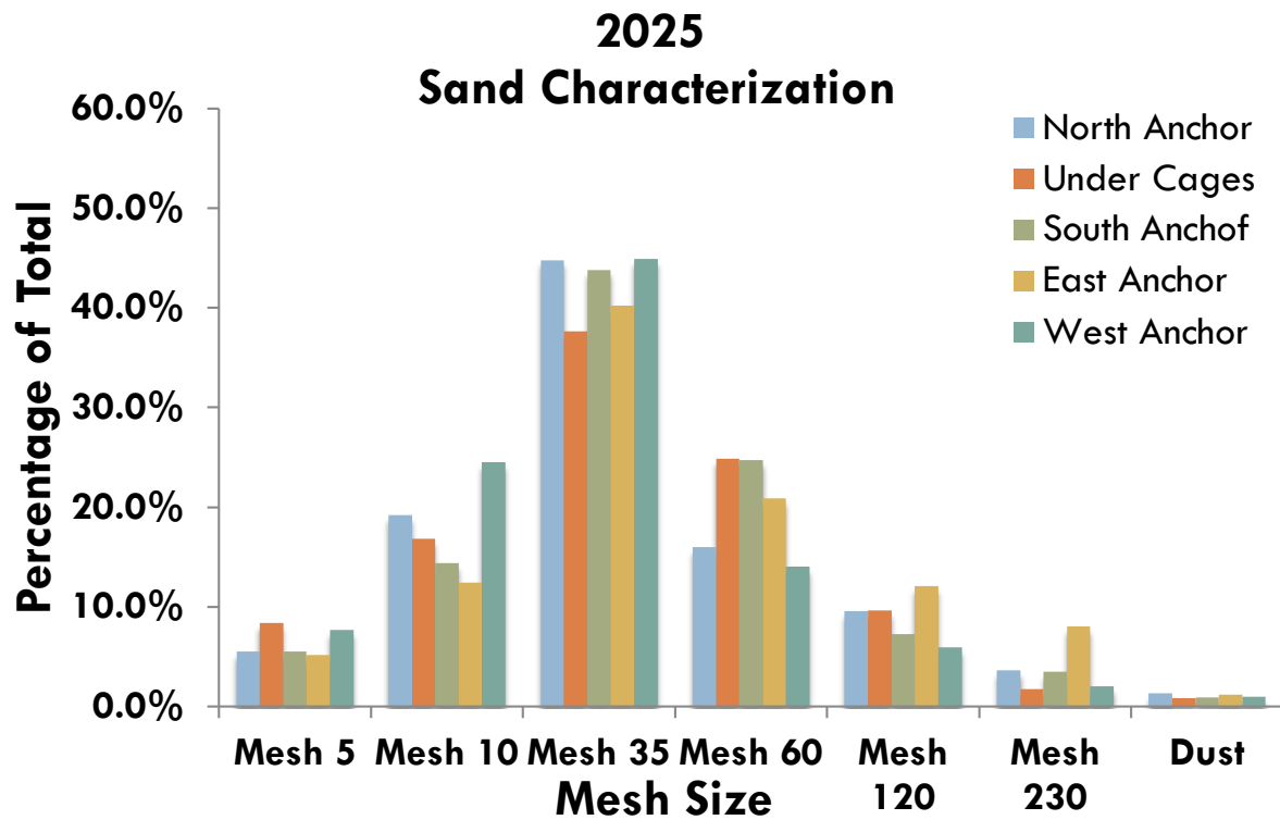
Figure 3. Sand characterization data for all sites from 2025 benthic analysis.
